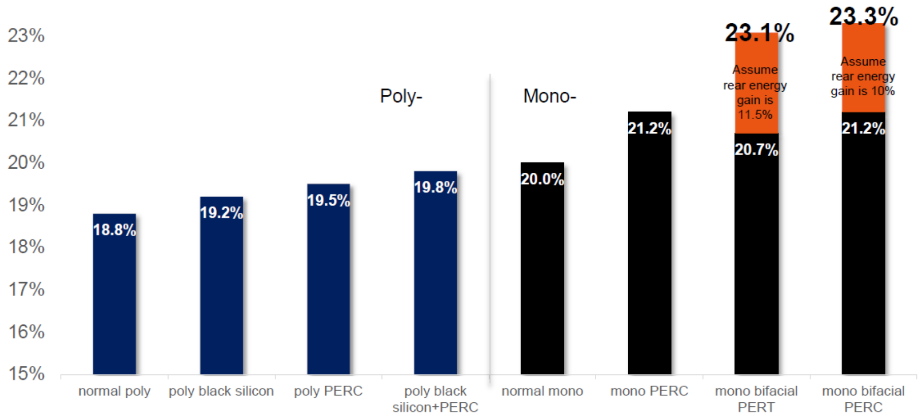
PV cell efficiency in Mainstream Market
